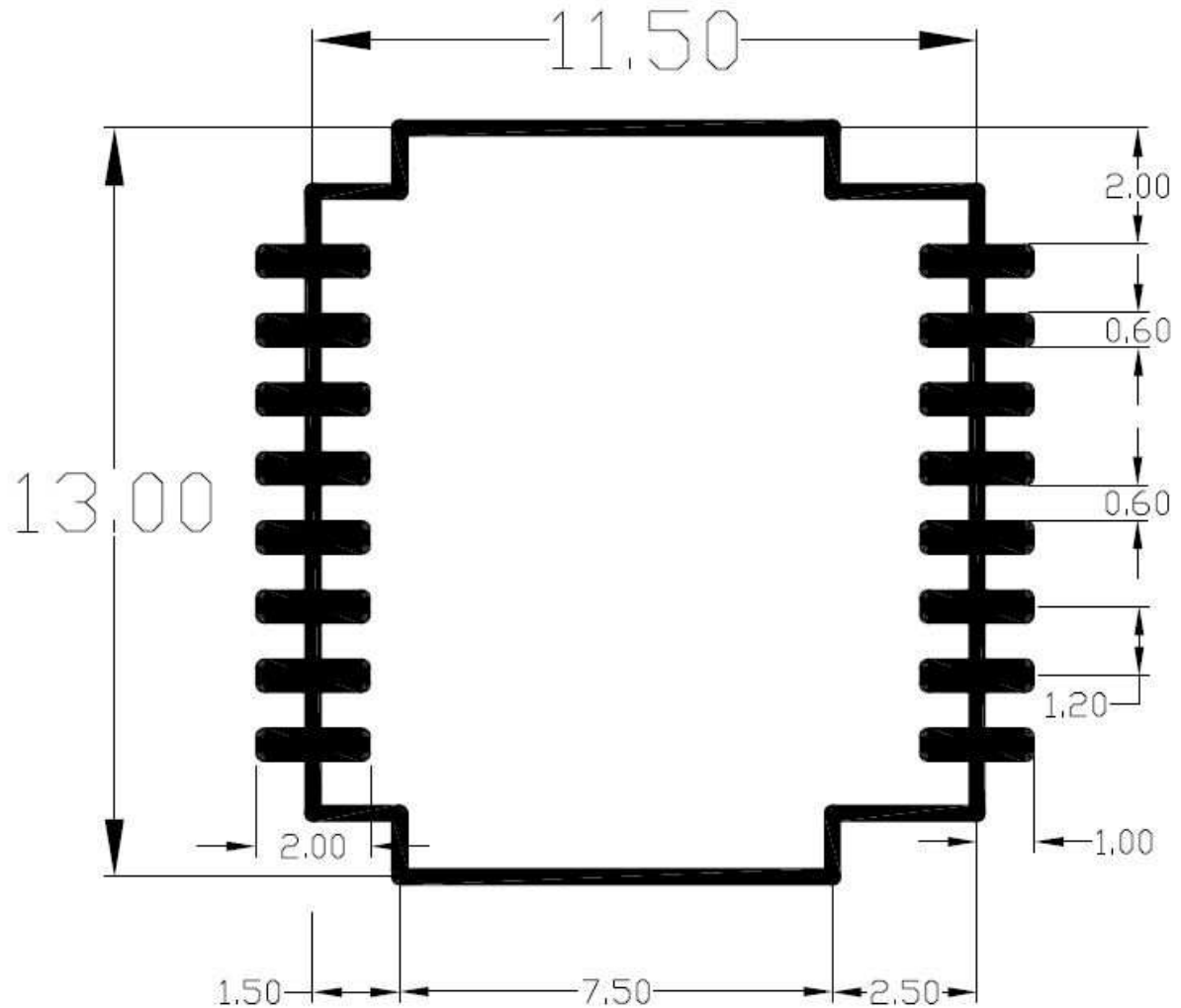
(Top view)
